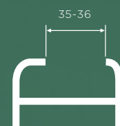
Žlijeb krila grilje Shutter sash groove
